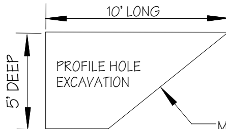
PROFILE VIEW
