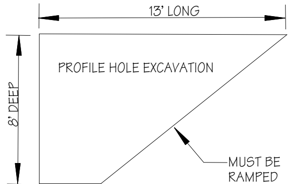
PROFILE VIEW
